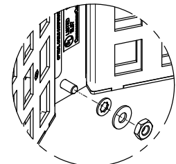
GROUNDING LUG with HARDWARE
