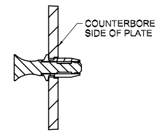
DETAIL A GROMMET/PLUNGER ORIENTATION
