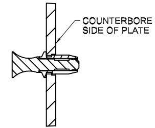
DETAIL A GROMMET/PLUNGER ORIENTATION
