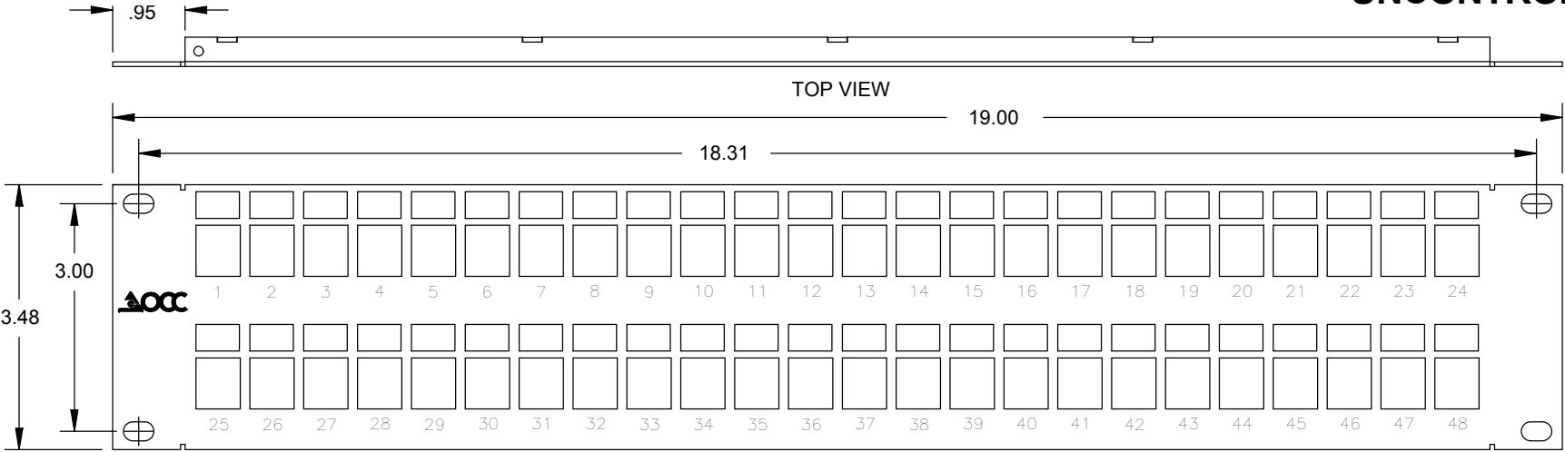
PATCH PANEL (OCC P/N AK48H)
