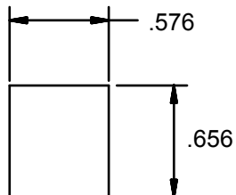
FACEPLATE, KMJ STYLE PORT DIMENSIONS
