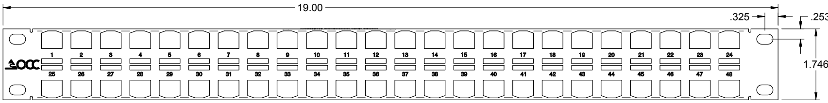
PATCH PANEL (OCC P/N AK481U)
