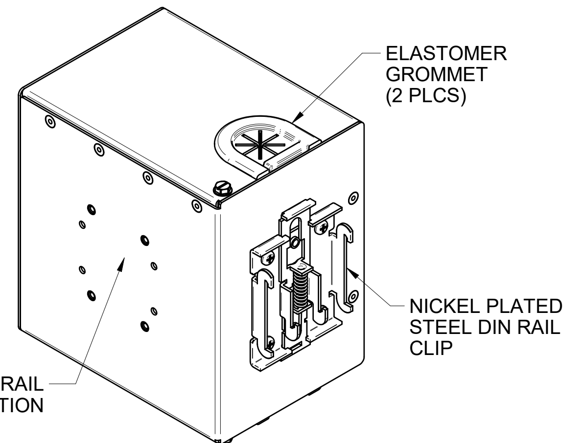
REAR ISOMETRIC VIEW
