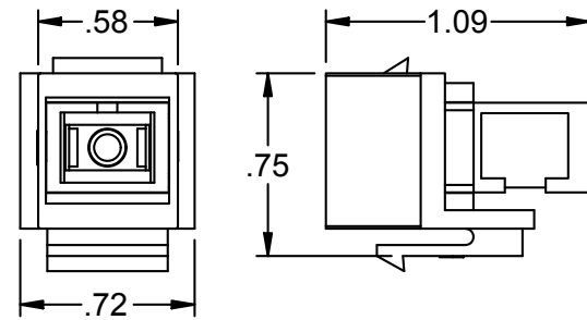
ASSEMBLY VIEW
