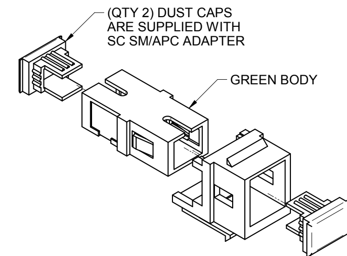
ISOMETRIC (EXPLODED)
