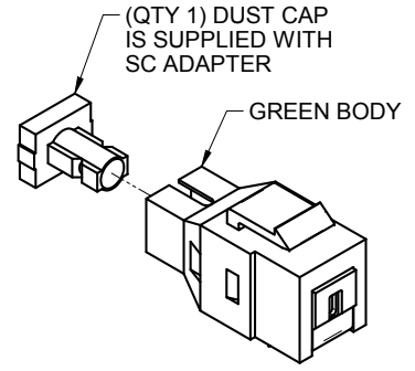
ISOMETRIC (EXPLODED)
