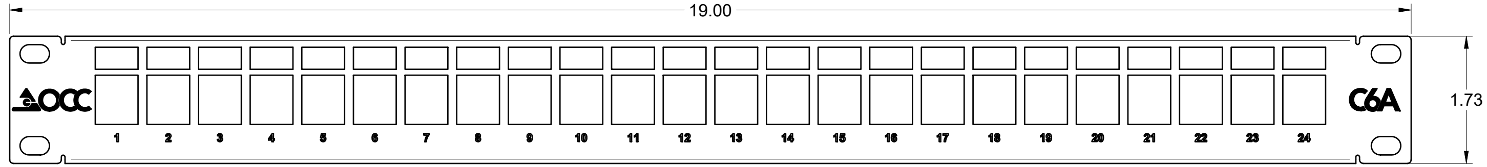
FRONT VIEW
