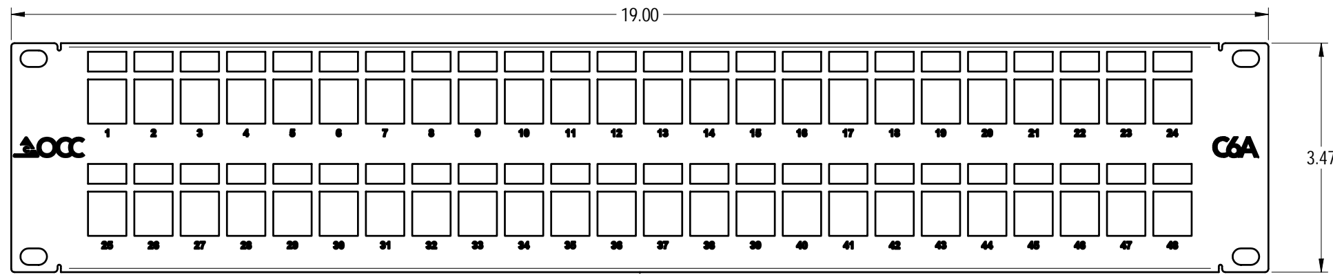
FRONT VIEW
