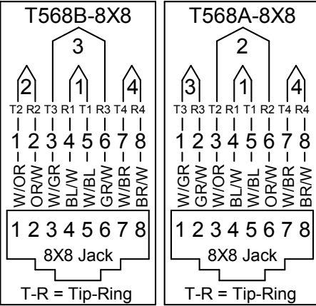
8 POSITION MODULAR JACK
