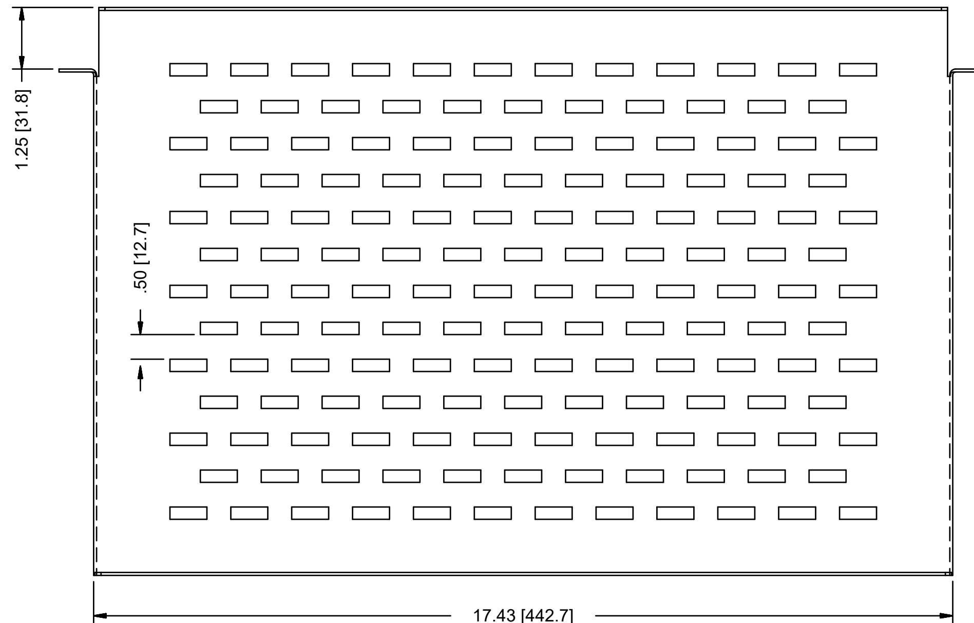
BOTTOM VIEW
