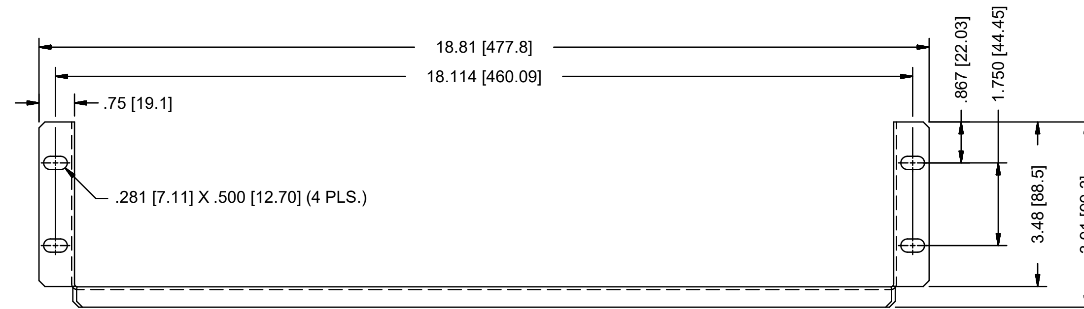
FRONT VIEW
