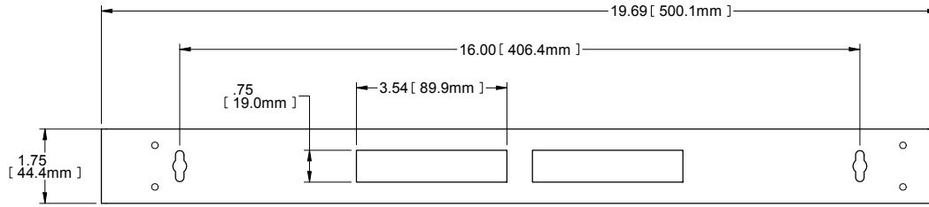
REAR VIEW
