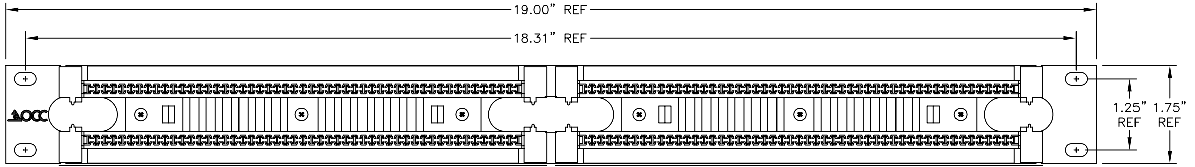
TOP VIEW
