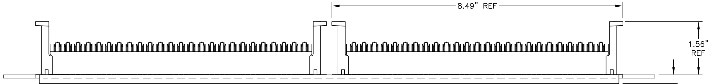
FRONT VIEW DCC100/110EFSRK SHOWN
