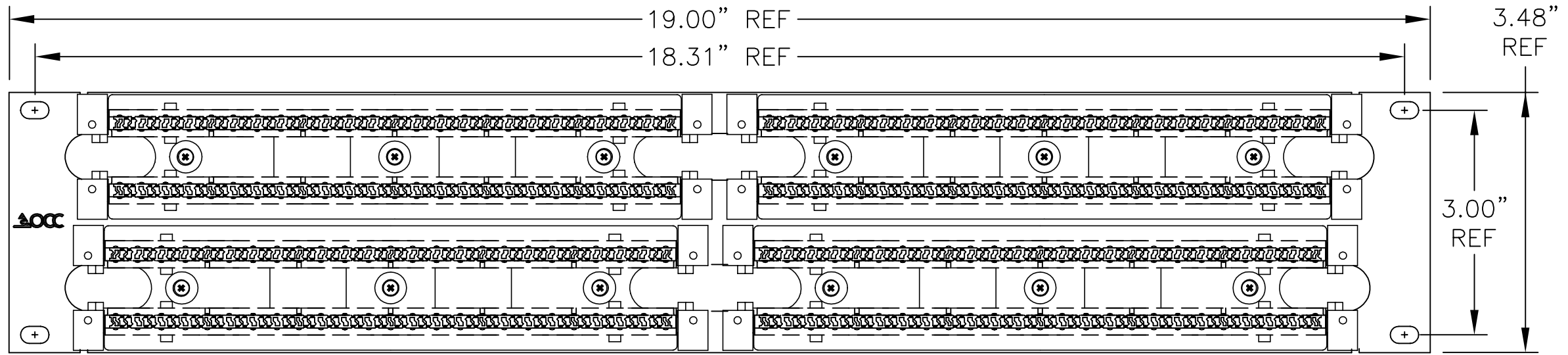
TOP VIEW
