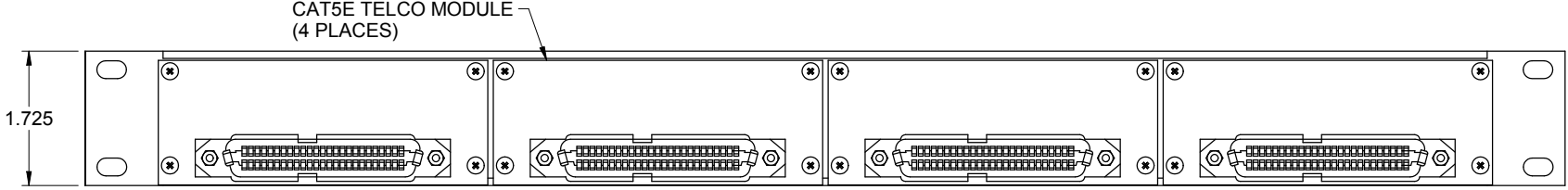
BACK VIEW (ROTATED 180° DEGREES) 24 PORT PATCH PANEL
