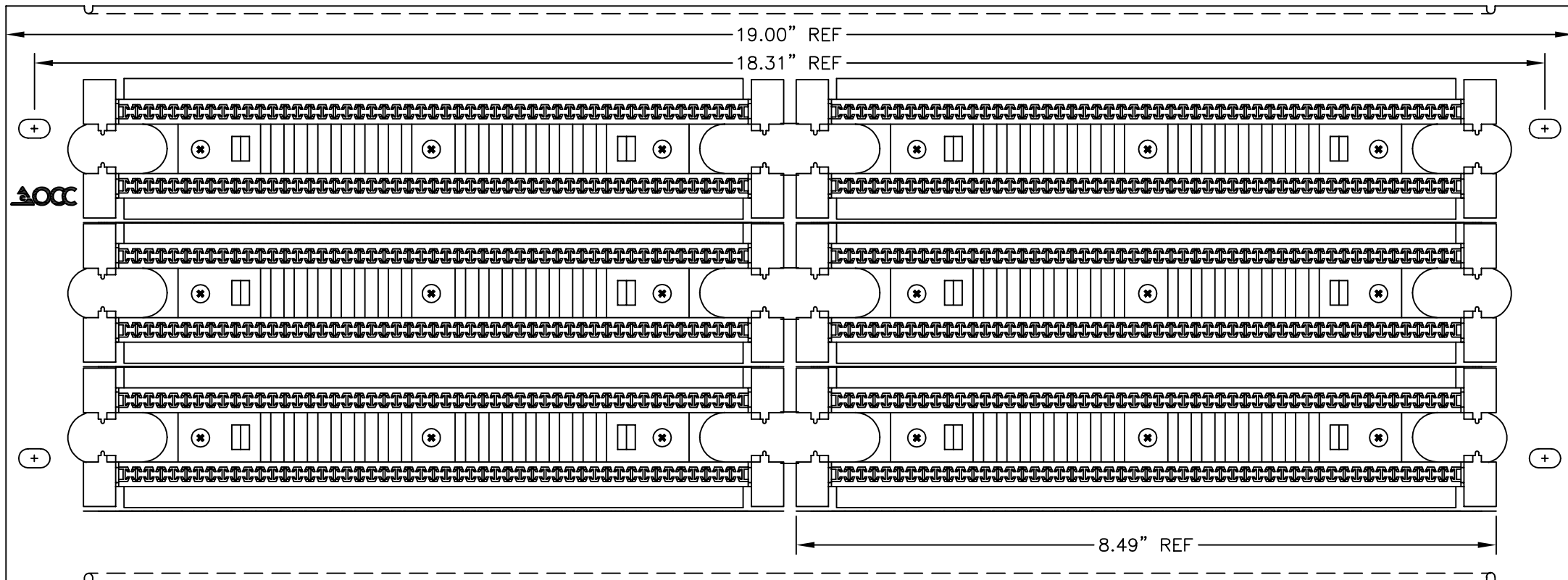
TOP VIEW
