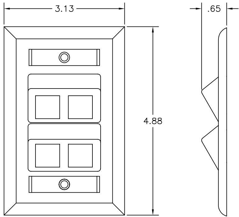
FRONT VIEW SINGLE-GANG WITH CLEAR PLASTIC WINDOWS
