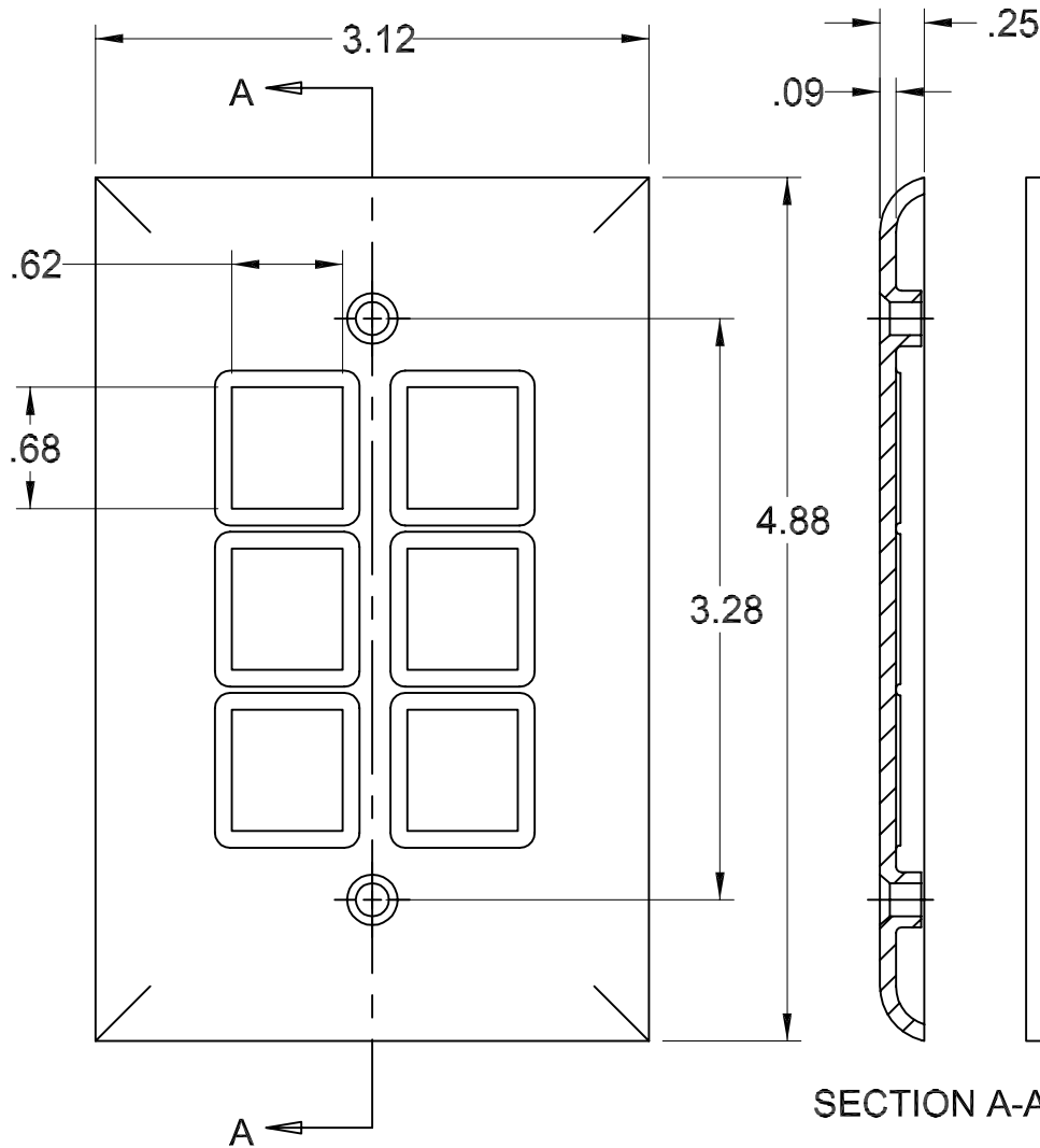
FRONT VIEW
