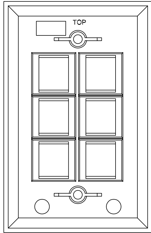
REAR VIEW
