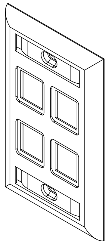
ISOMETRIC (FRONT)
