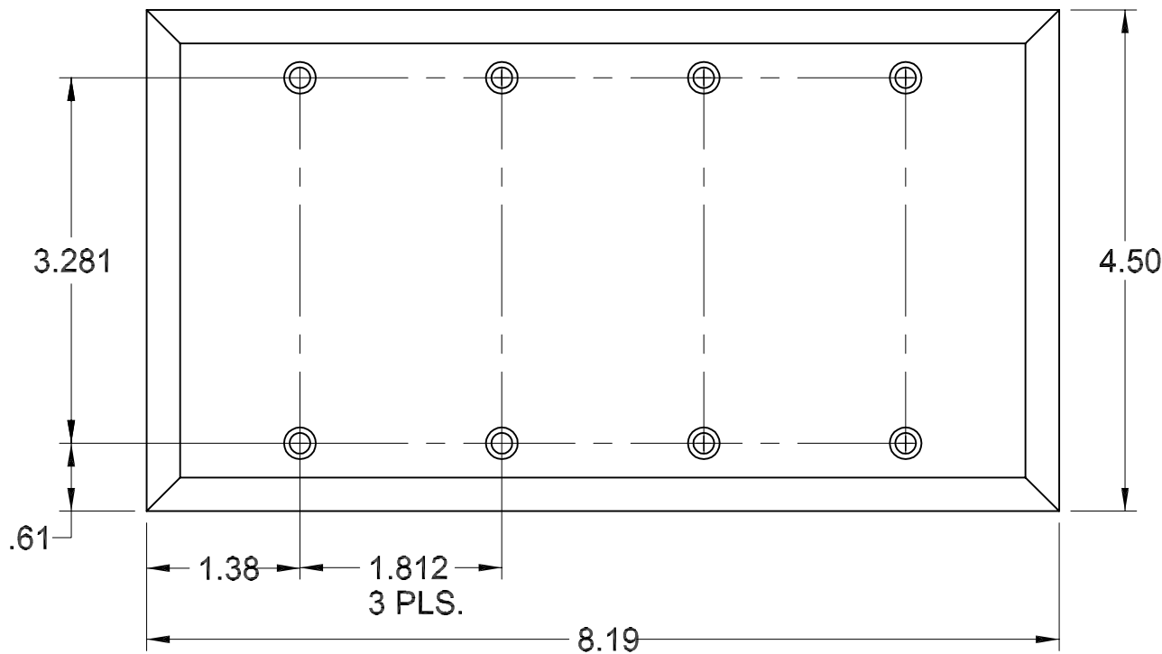
FRONT VIEW (FACEPLATE ONLY)
