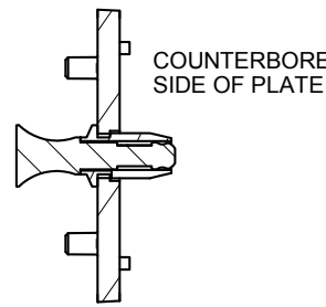
DETAIL A GROMMET/PLUNGER ORIENTATION
