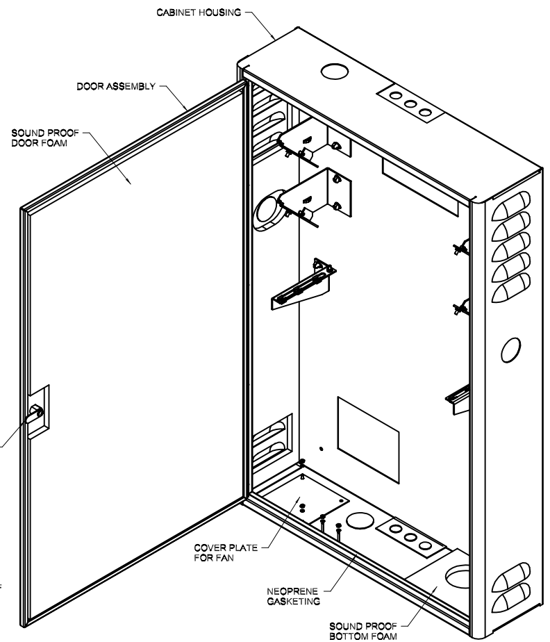
ISOMETRIC VIEW
