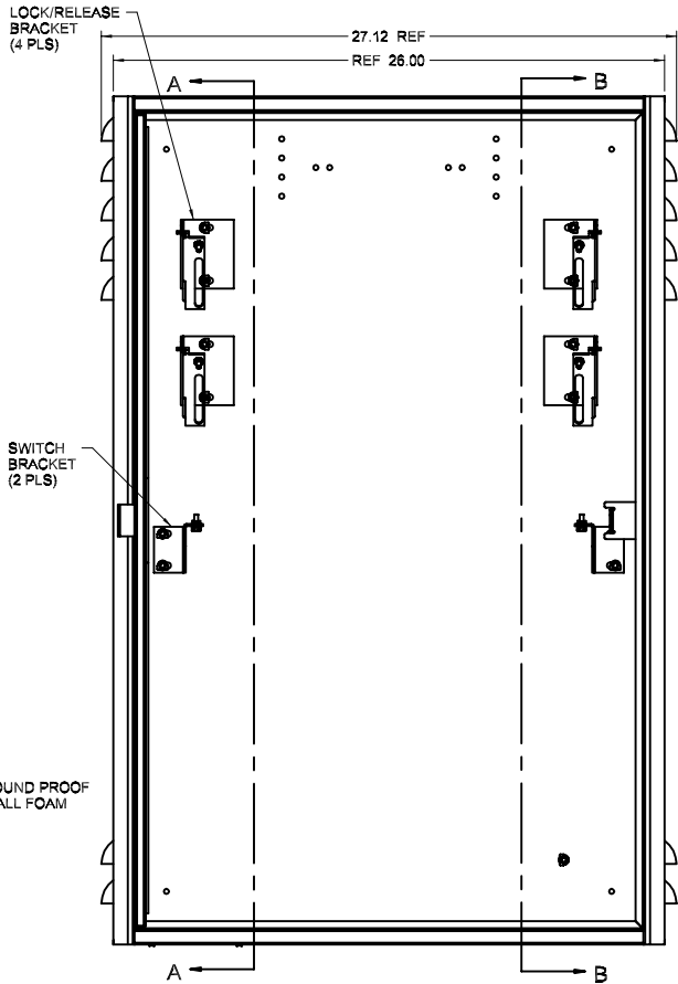
FRONT VIEW (OPENED)
