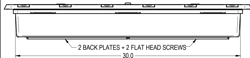
SIDE VIEW
