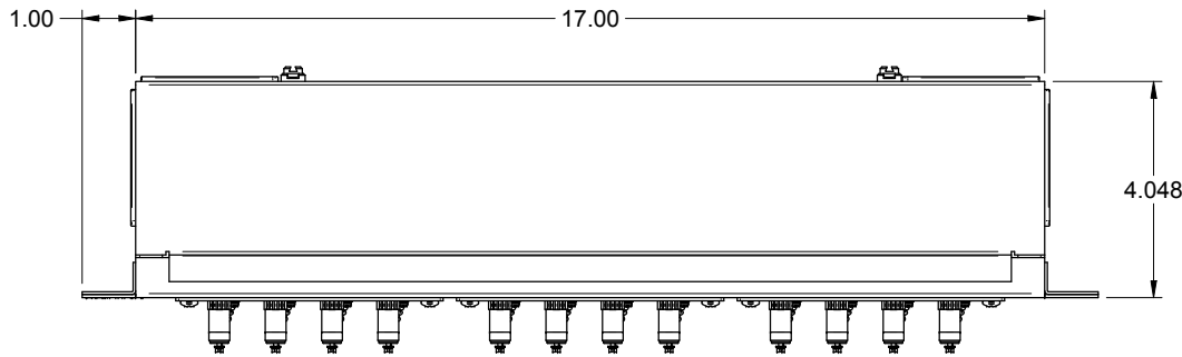
TOP VIEW
