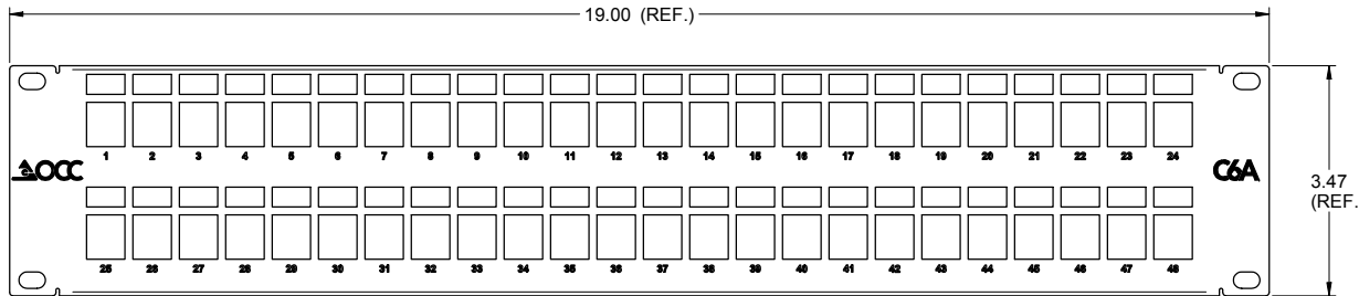
FRONT VIEW AK48STP6A
