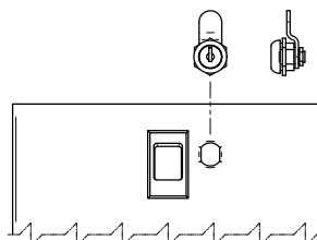
INNER DOOR/WORK SHELF LOCKABLE DOOR LATCH (OPTIONAL)
