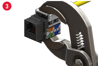
STUFFER CAP TERMINATION METHOD
