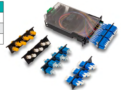
OCC Fiber Splice Cassette with Fiber Adapter Plates
