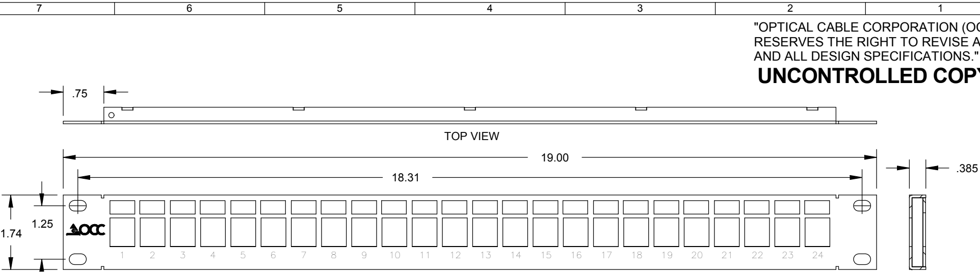
PATCH PANEL (OCC P/N AK24)
