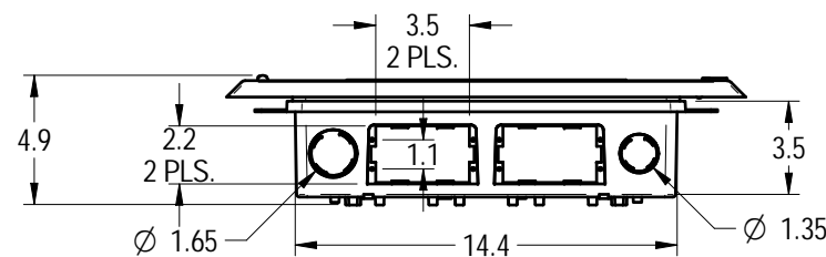
BOTTOM VIEW
