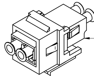
COMPLETED ASSEMBLY OCC p/n AKDLCSxx
