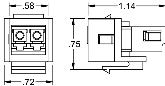
ASSEMBLY VIEW
