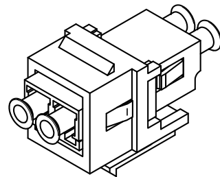
COMPLETED ASSEMBLY
