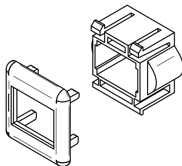
EXPLODED VIEW (SHOWN FOR CLARITY) ISOMETRIC VIEW P/N AADLCAxx
