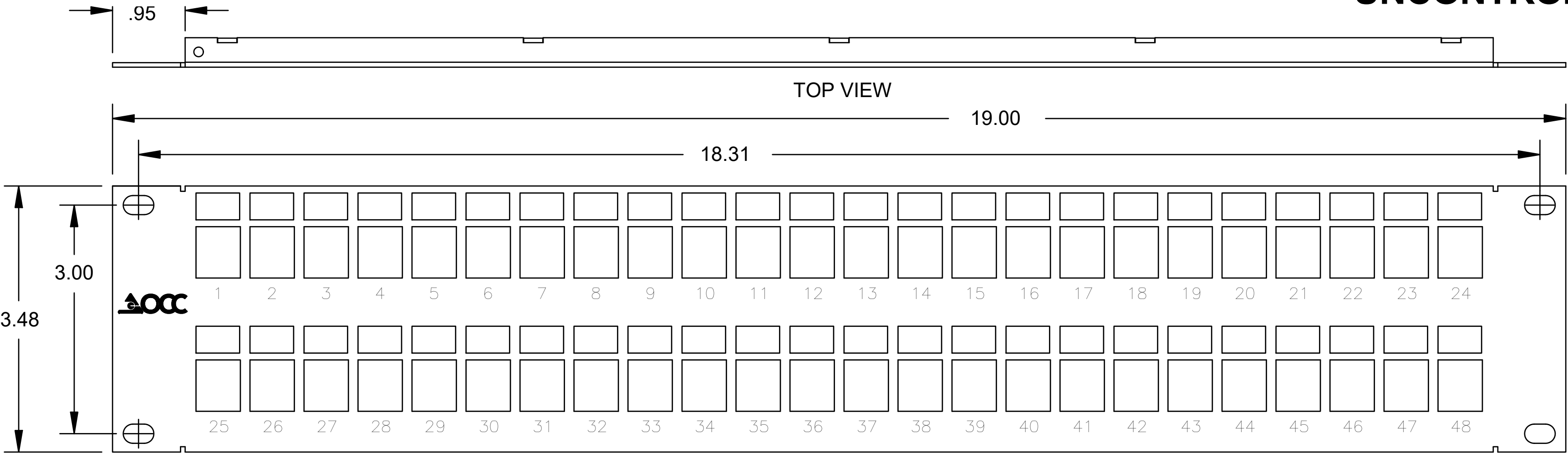
PATCH PANEL (OCC P/N AK48H)
